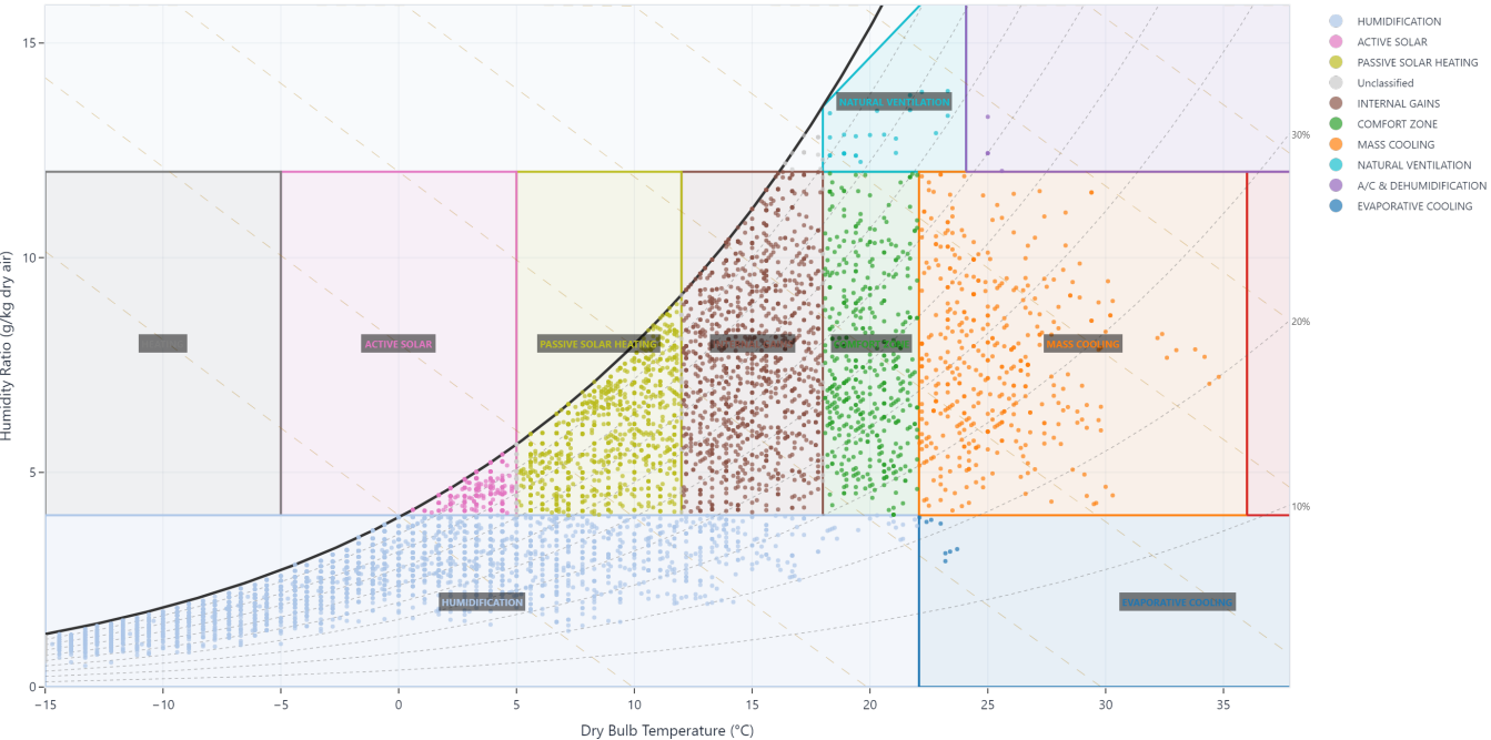
Psychrometric Chart – ASHRAE Style
